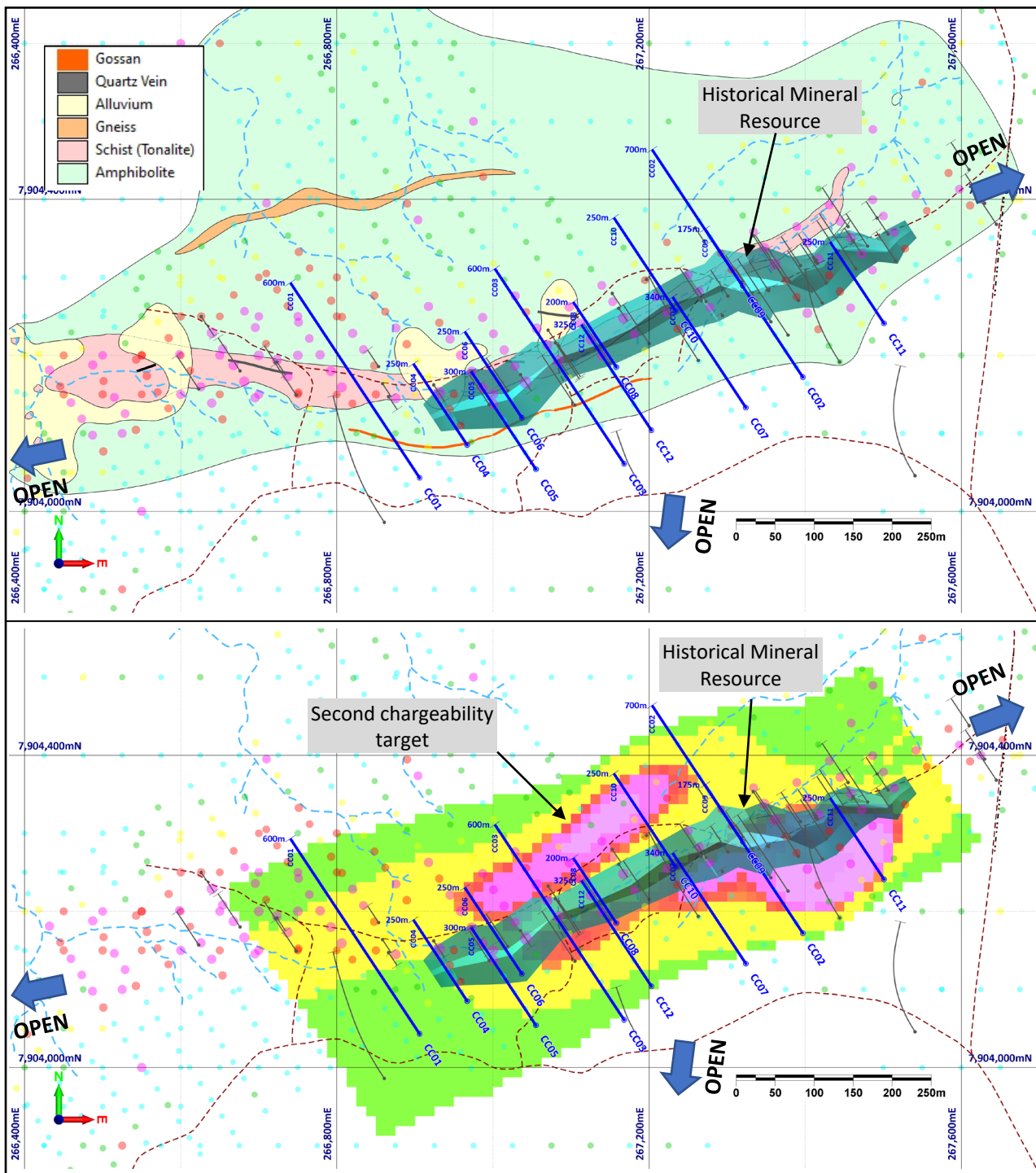
Figure 12. Plan views of Cockie Creek Prospect surface geology (top) and IP chargeability data (bottom). Gridded soil copper geochemistry, planned drill holes (blue traces) and wireframe of the historical Mineral Resource are shown in each plan.
