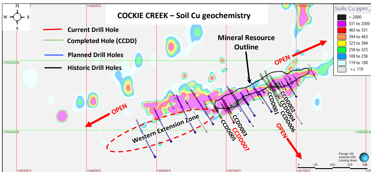
Figure 9. Gridded soil Cu geochemistry of the Cockie Creek area showing the Western Extension Zone, outline of historical Mineral Resource and current program drill holes.
