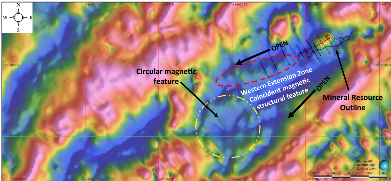
Figure 10. Aerial magnetic image (RTP) of the Cockie Creek regional area showing the outline of the historical Mineral Resource and the Western Extension Zone (red polygon) as supported by a linear series of magnetic features. A prominent large circular magnetic feature is located south of the Western Extension Zone (yellow circle).
