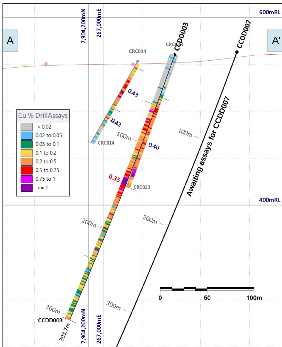
Figure 3. Cross-section (+/- 20m) taken along A-A' (as shown in Figure 2) looking east-northeast showing CCDD003 and historic CRC023 (twinned), proximal historic drill hole CRC014, and the trace of CCDD007 from the current program (assays pending). Down-hole copper assay values (1m intervals) are represented as grade categories.
