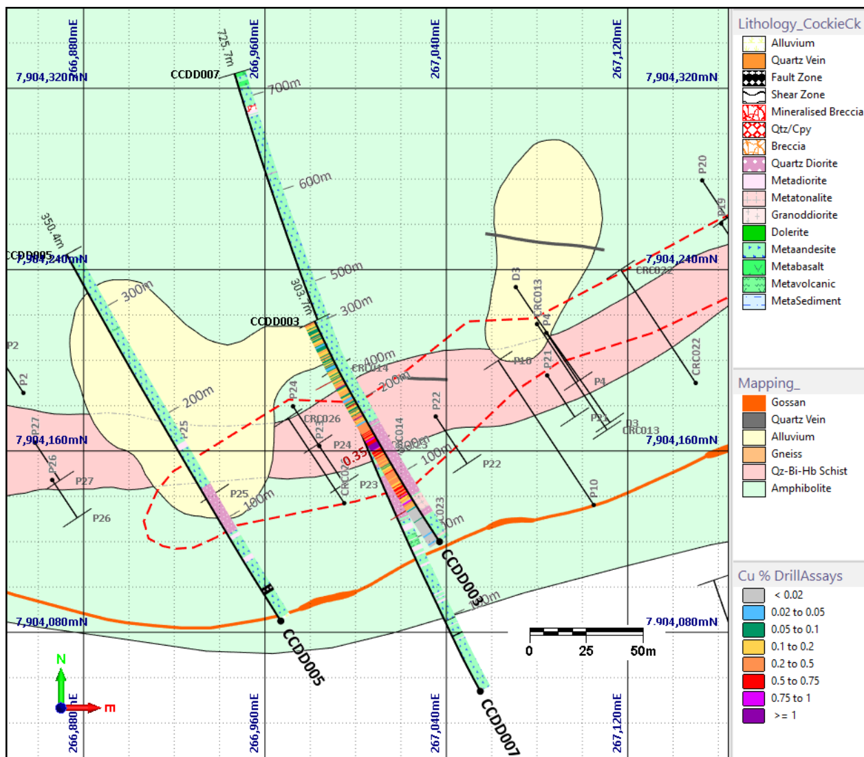
Figure 4. Plan geological map of Cockie Creek showing drill holes from the current program with assay data (CCDD003) and lithologies from core logging. Note: only lithology is shown for CCDD005 and CCDD007. Note the long Cu intersection with good Cu grades within meta-andesite wall rocks that extend to the end of CCDD003.
