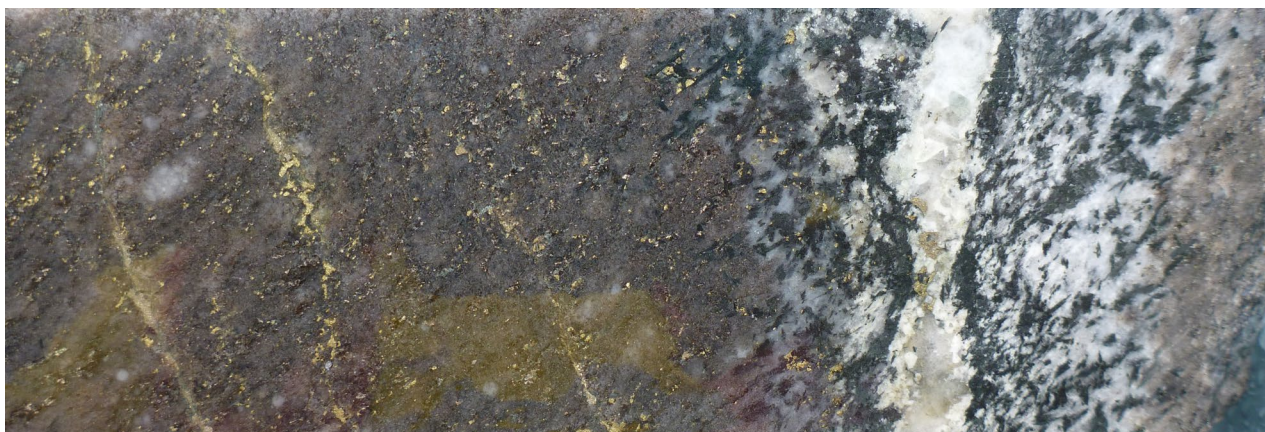
Figure 8. Core from CCDD003 (85.5 m) with a deformed 1 cm wide quartz-pyrite-chalcopyrite-molybdenite vein surrounded by a zoned sodic-calcic alteration selvage consisting of dark green actinolite (inner) and greyish white albite and quartz (outer). The vein crosscuts well foliated and potassic altered (biotite) quartz diorite that is cut by narrow (1-5 mm wide) “stringer” veins of pyrite-chalcopyrite ± pyrrhotite. Such features are characteristic of “D veins” in porphyry copper-gold-molybdenum deposits. Note the alignment of brown flakes of hydrothermal biotite and sulphide mineral within the foliation. Interval contains 0.71% Cu, 0.12 g/t Au, and 164 ppm Mo.
