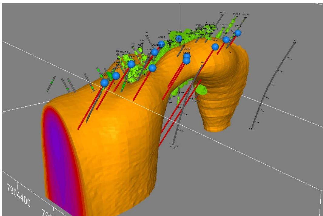
Figure 11. 3D IP chargeability model showing moderate to high chargeability zone. Historical drill holes (grey traces) and copper mineralisation (green) with 2023 planned drill holes in red. Viewed looking northeast.
