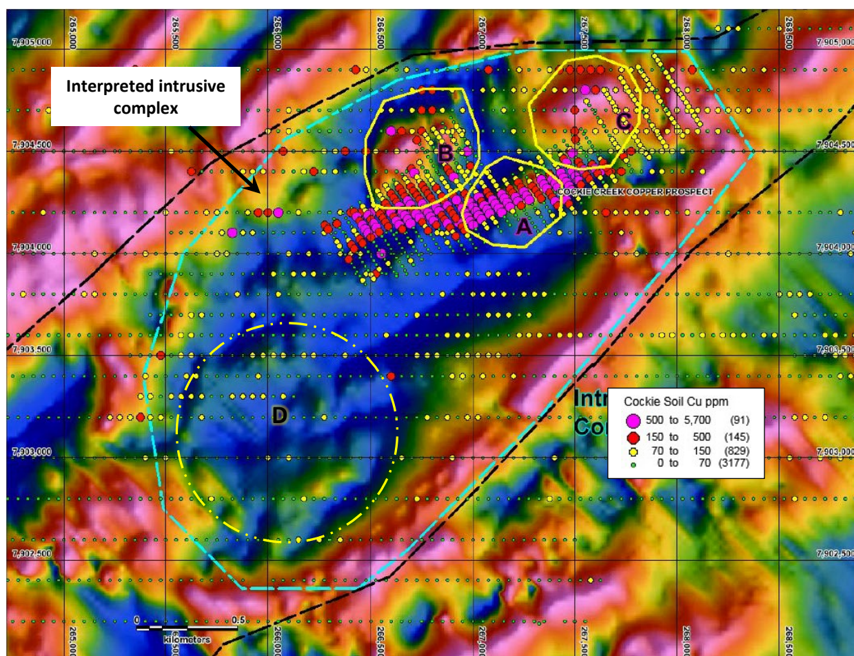
Figure 13. Cockie Creek thematic Cu soil data and interpreted porphyries on TDr VI NSSF processed airborne magnetics data, showing interpreted porphyry intrusions (A to D) within an interpreted intrusive complex.
