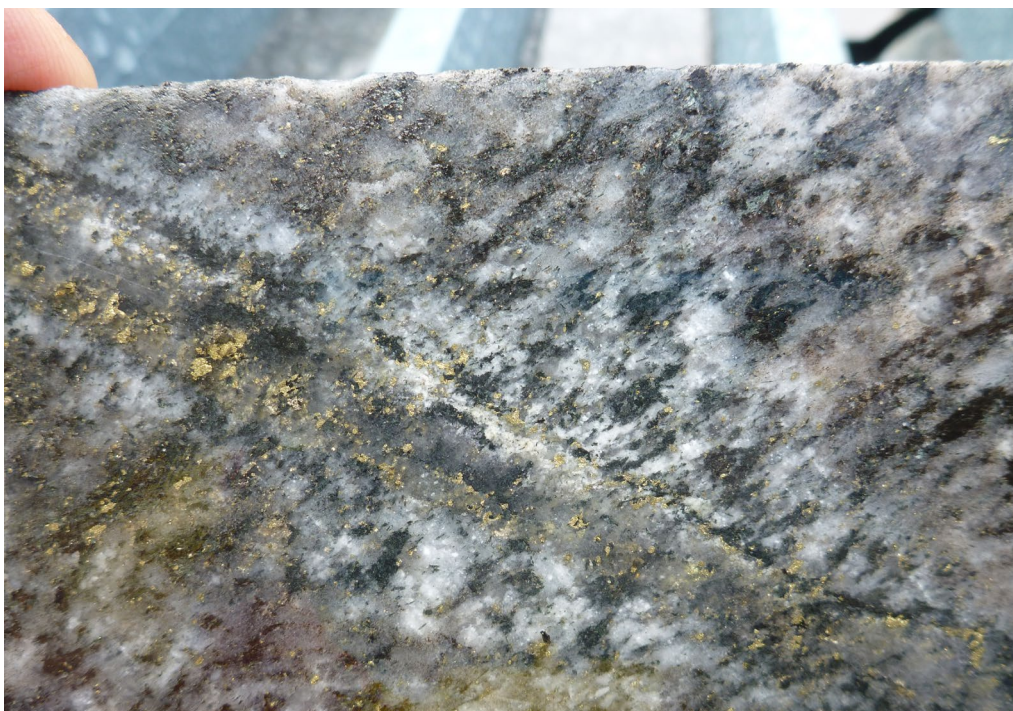
Figure 7. Core from CCDD003 (93.7 m) with a 1 cm wide quartz-pyrite-chalcopyrite-pyrrhotite-molybdenite vein crosscutting foliation in a quartz diorite. The vein is surrounded by an alteration selvage of dark green actinolite and milky white albite (sodic-calcic alteration) that preferentially extends along the foliations and replaces pale brown hydrothermal biotite (potassic alteration). Despite the deformation and partial recrystallisation, discrete wall-rock parallel bands of sulphide minerals are preserved indicating multiple open-space vein-filling events and extensional “crack-seal” vein growth. These features are characteristic of “ B veins ” in porphyry copper-gold-molybdenum deposits. Interval contains 0.24% Cu, 0.06 g/t Au, and 33 ppm Mo.
