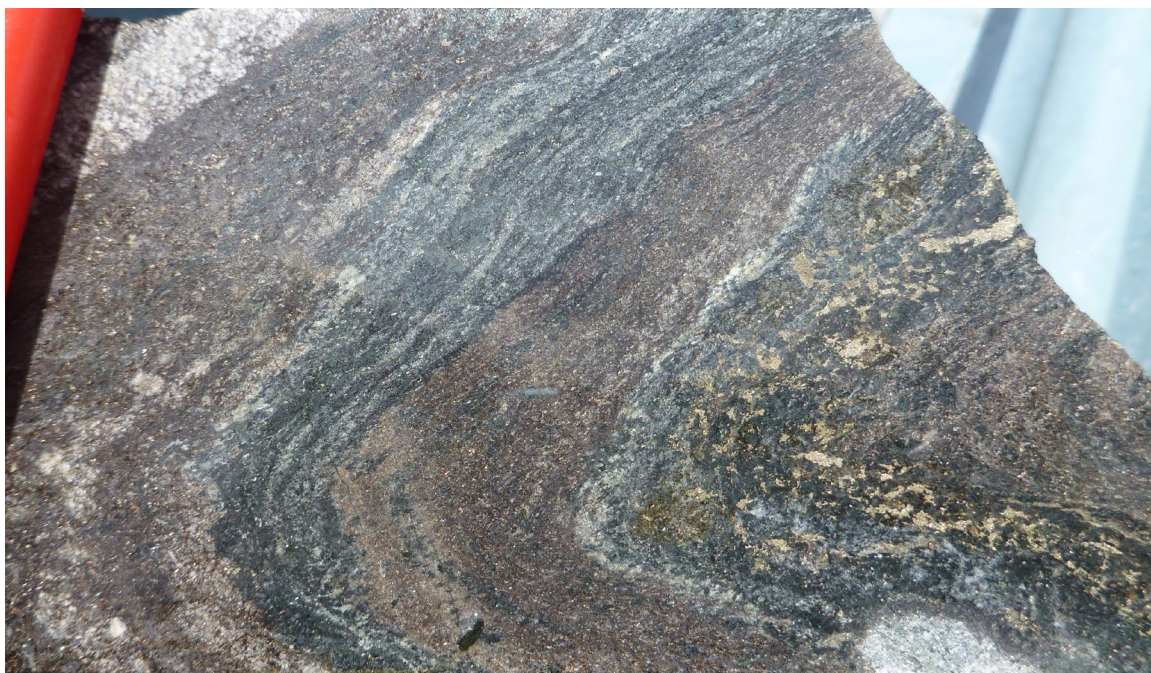
Figure 5. Core from CCDD003 (52.5 m) of folded meta-andesite. Narrow foliated bands of pale brown biotite (potassic alteration) alternate with dark green bands of actinolite and milky white albite (sodic-calcic alteration) associated with brassy yellow pyrite-chalcopyrite and minor quartz. The folded alteration bands suggest that potassic alteration, sodic-calcic alteration and sulphide mineralisation pre-date the folding event. Original quartz-sulphide vein textures, if present, have been destroyed. Interval contains 0.02% Cu.
